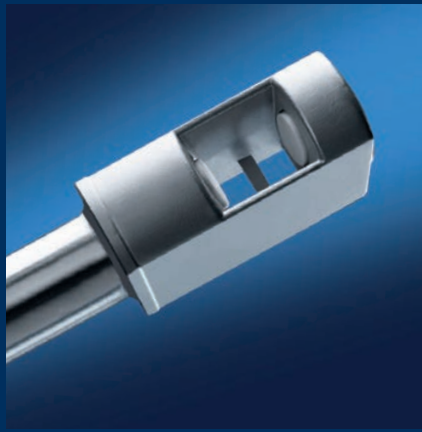
Vortex Flow Sensor VA as insertion probe
