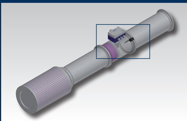
ExactFlow II in a customer-specific application with multiphase flow straightener. 3D drawings for spatial overview.
