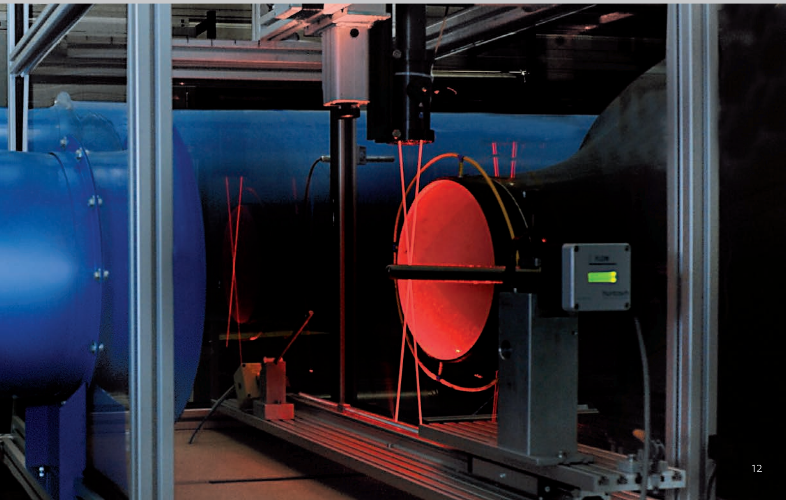
Wind tunnel with laser Doppler anemometer reference 0.15 ... 70 m/s
